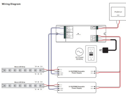
Wiring Diagram
