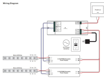
Wiring Diagram
