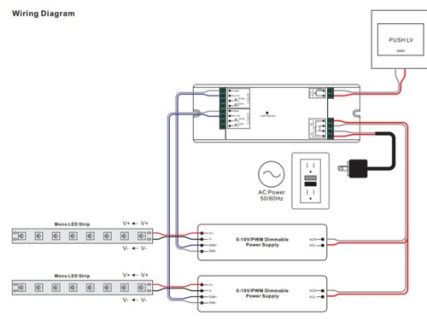
Wiring Diagram
