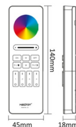
Remote
