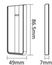
Remote Holder
