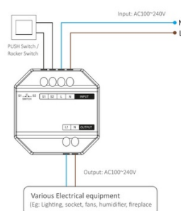
Connection Diagram
